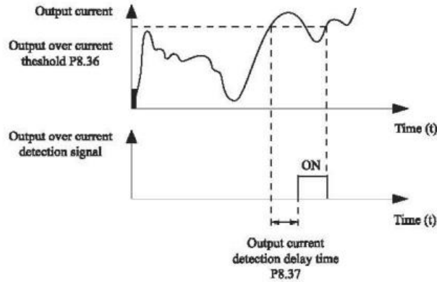
Figure 4-20 Output over current detection
