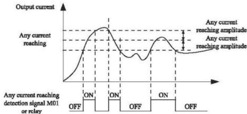
Figure 4-21 Any current reaching detection
