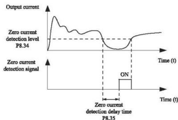
Figure 4-19 Zero current detection
