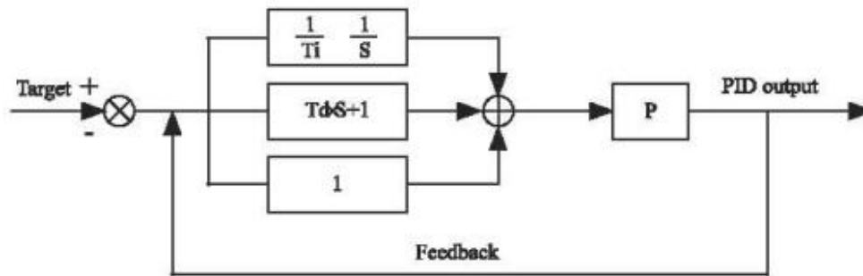
Figure 4-23 Principle block diagram of PID control
