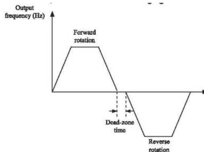
Figure 4-13 Forward/Reverse rotation dead-zone time
