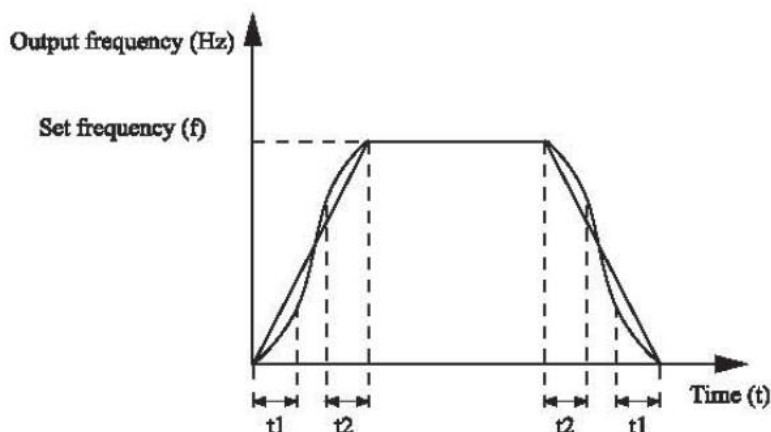
Figure 4-2 S-curve acceleration/deceleration A
