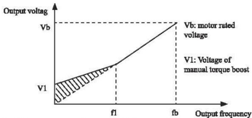
Figure 4-5 Manual torque boost
