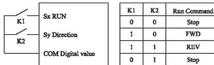
Figure 4-9 Setting of two-line mode 1
