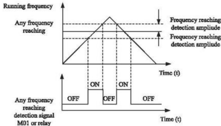
Figure 4-18 Any frequency reaching detection
