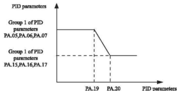
Figure 4-24 PID parameters switchover
