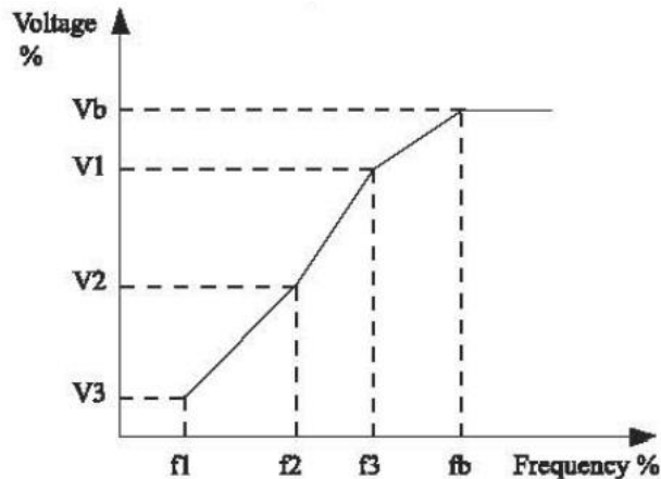
Figure 4-6 Setting of multi-point V/F curve
