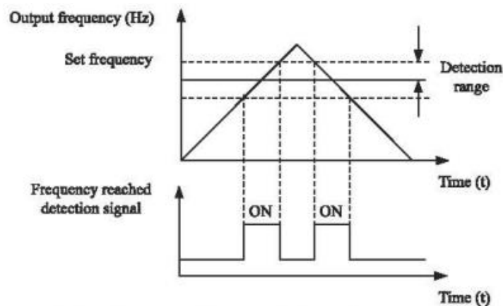
Figure 4-15 Detection range of frequency reached
