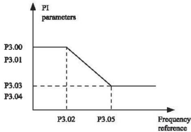
Figure 4-4 Relationship between running frequency and PI parameters
