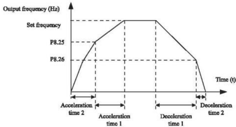
Figure 4-17 Acceleration/deceleration time switchover
