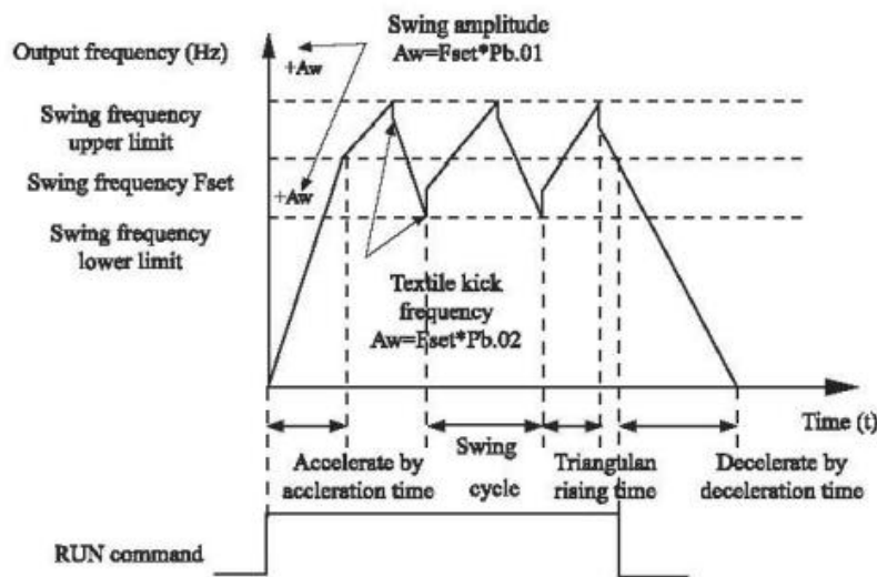
Figure 4-26 Swing frequency control
