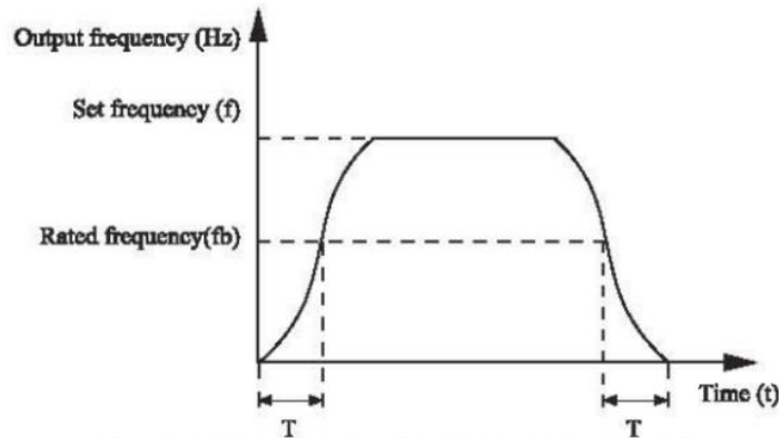
Figure 4-1 S-curve acceleration/deceleration B
