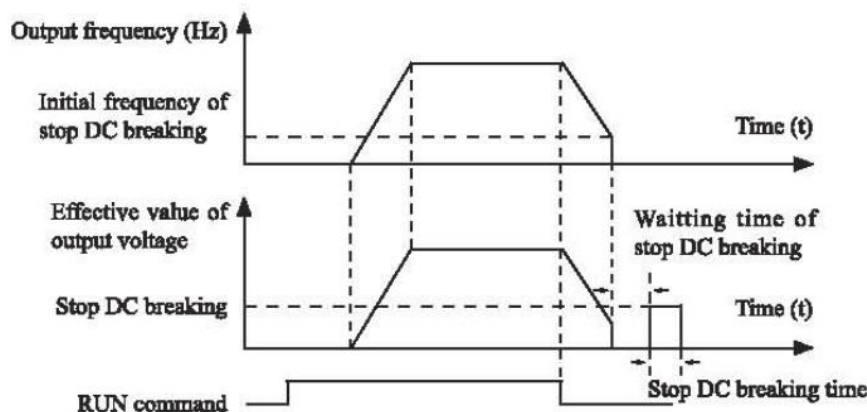
Figure 4-3 Stop DC braking process
