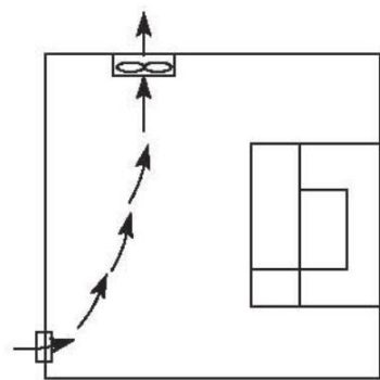
Incorrect installation position of the fan
