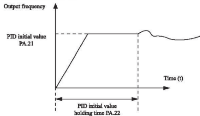
Figure 4-25 PID initial value function
