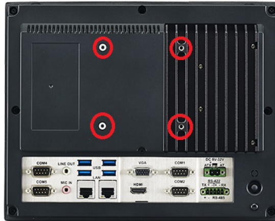
Figure 1.2 Rear Panel
